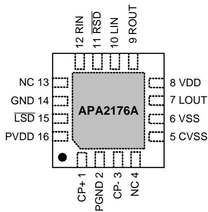
TQFN3x3-16 (Top View)
