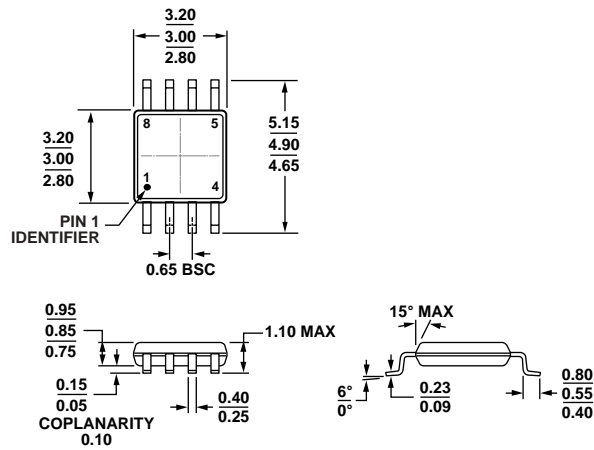
Figure 31. 8-Lead Standard Small Outline Package [SOIC_N] Narrow Body (R-8) Dimensions shown in millimeters and (inches)
