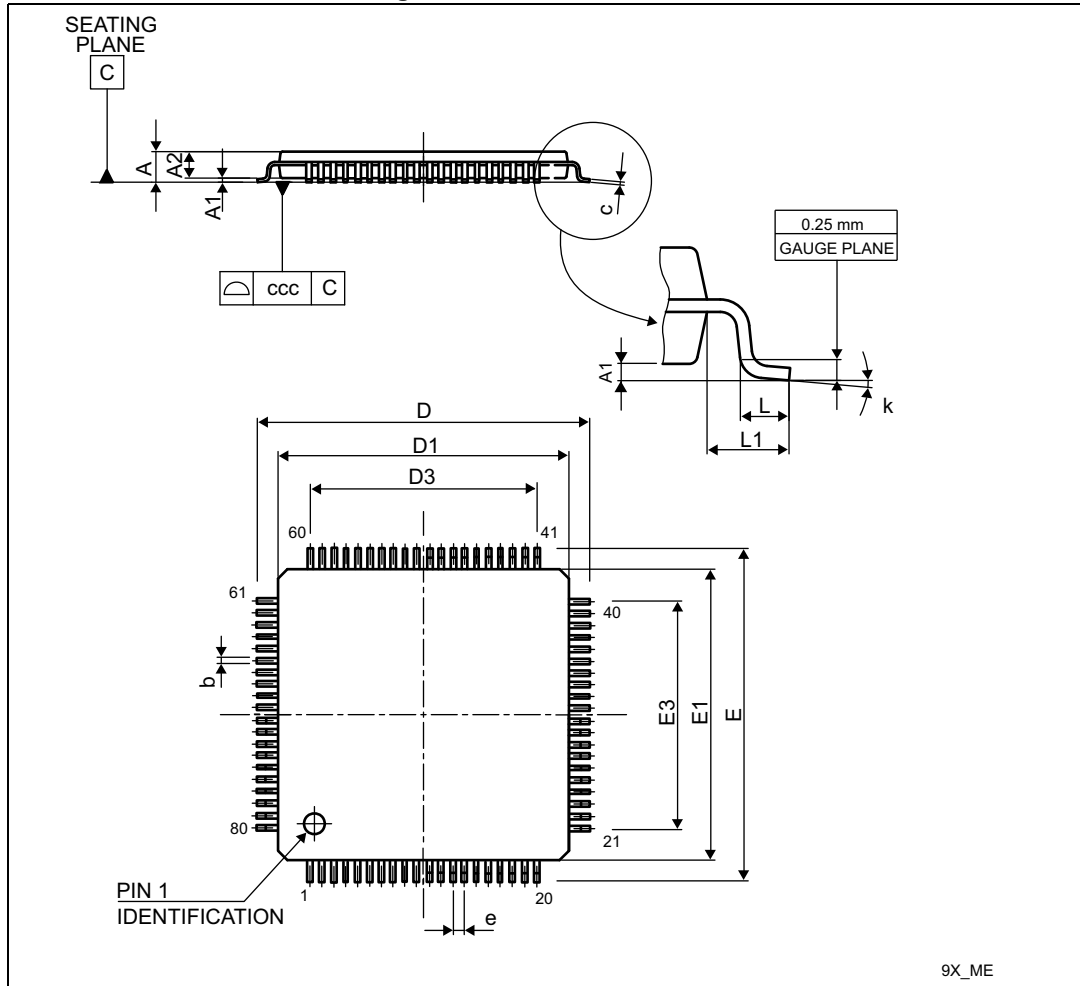
Figure 58. LQFP80 - Outline
