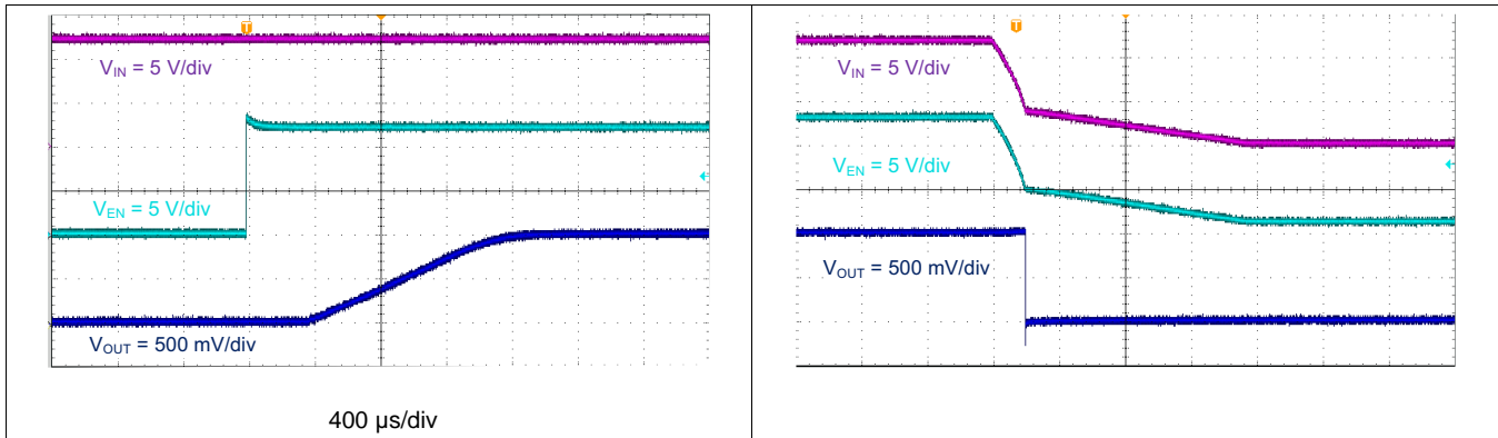
Figure 27. TPS564201 Startup Relative to EN
