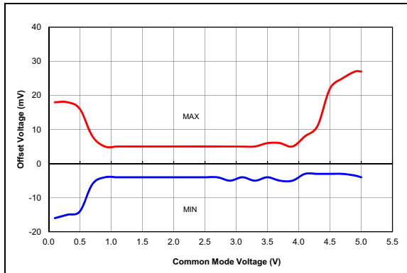
FIGURE 38-67: Comparator Offset, NP Mode ( CxSP = 1 ), V_{DD} = 5.5V , Typical Measured Values from -40^\circ C to 125^\circ C , PIC16F18855/75 Only.
