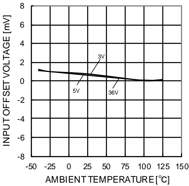
Figure 62. Input Offset Voltage - Ambient Temperature ( V_{ICM}=0V , OUT=1.4V )
