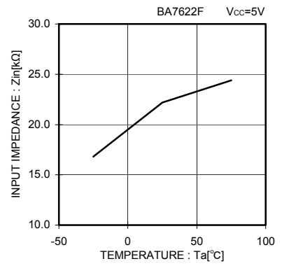
Fig.57 Input impedance vs. Temperature
