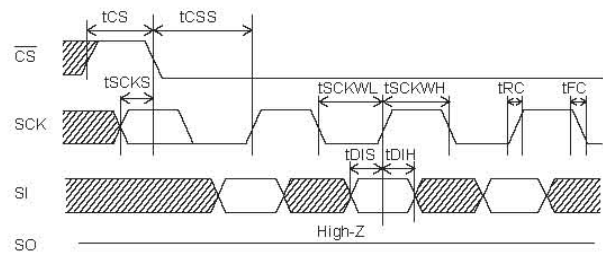
Figure 1. Input timing
