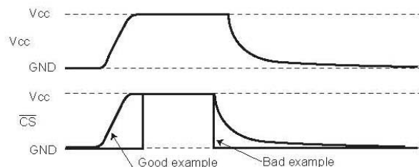
Figure 61. CS timing at power ON/OFF
