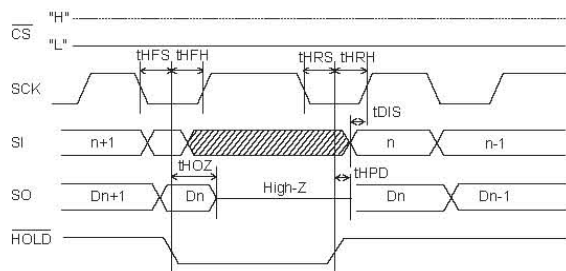
Figure 3. \overline{\text{HOLD}} timing
