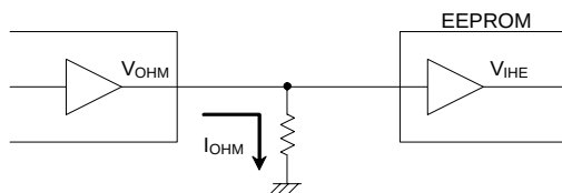
Figure 52. Pull down resistance
