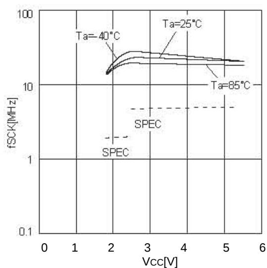
Figure 15. SCK frequency fSCK
