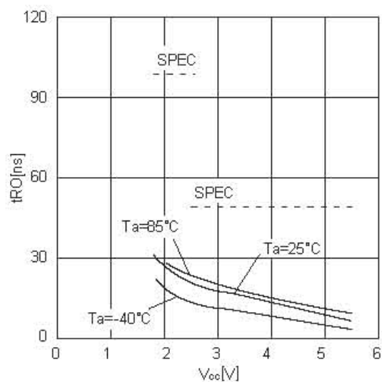
Figure 30. Output rise time tRO
