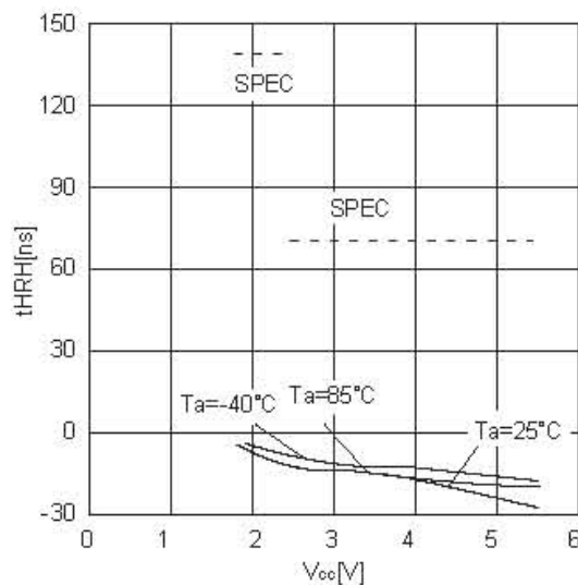
Figure 27. HOLD release hold time tHRH
