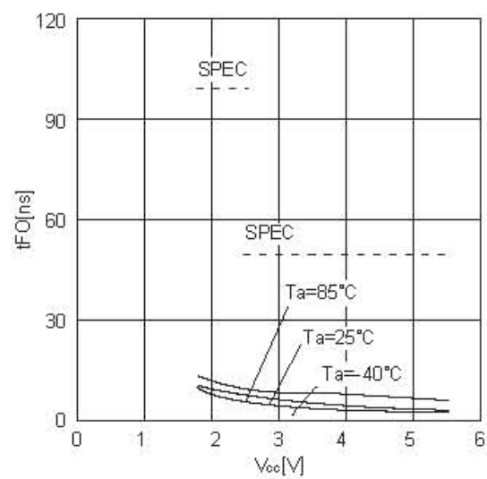
Figure 31. Output fall time
