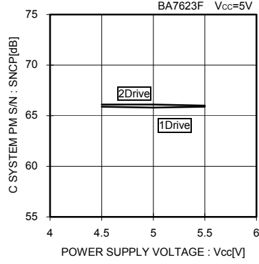
Fig.20 C system PM S/N vs. Supply voltage
