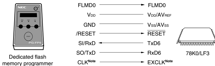
Figure 28-7. Communication with Dedicated Flash memory programmer (UART6)
