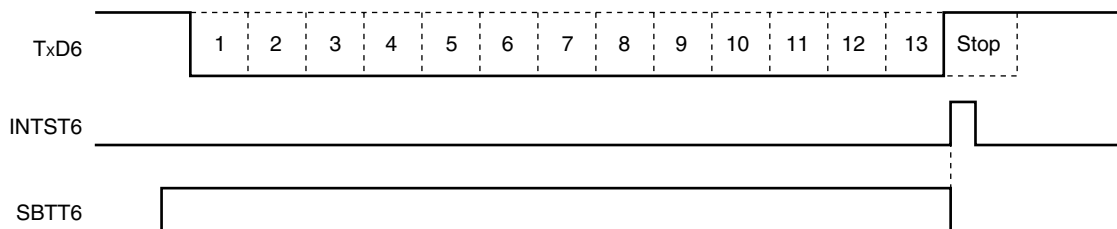
Figure 15-24. SBF Transmission
