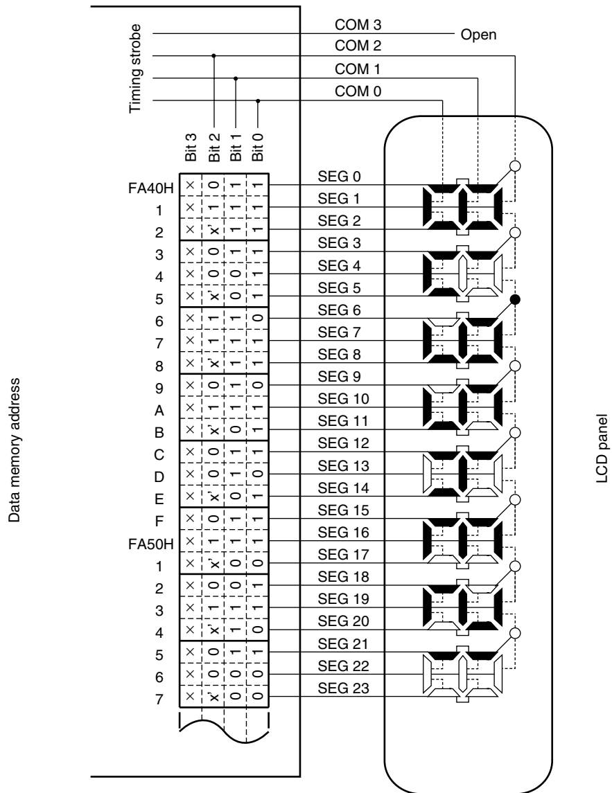
Figure 18-24. Example of Connecting Three-Time-Slice LCD Panel
