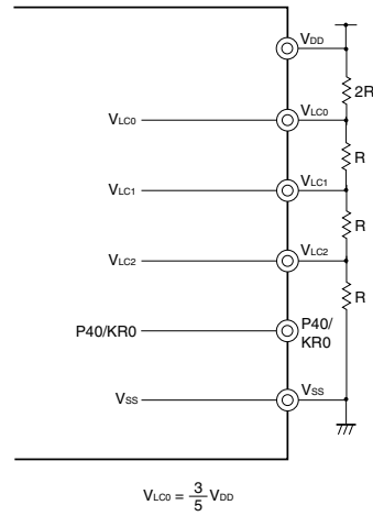
(f) 1/3 bias method (MDSET1, MDSET0 = 0, 0) (example of V_{DD} = 5\text{ V} , V_{LC0} = 3\text{ V} )
