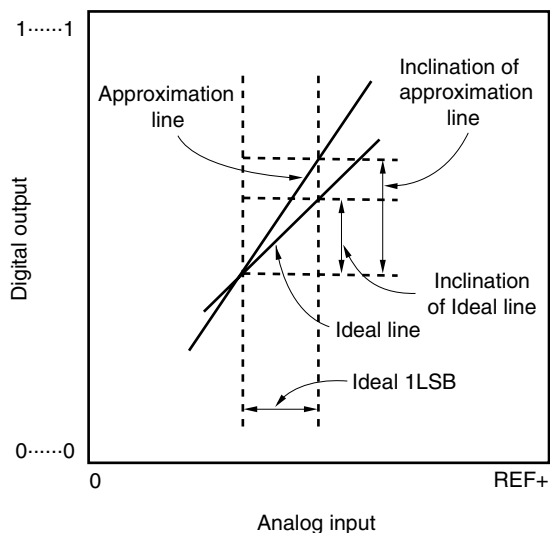
Figure 13-18. Gain Error
