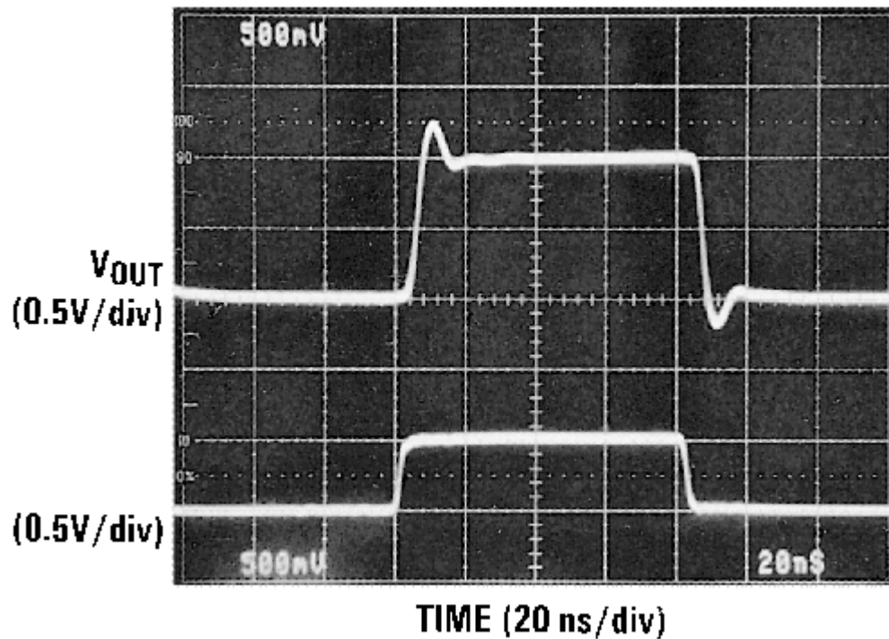
Figure 80. R_f = 820\Omega
