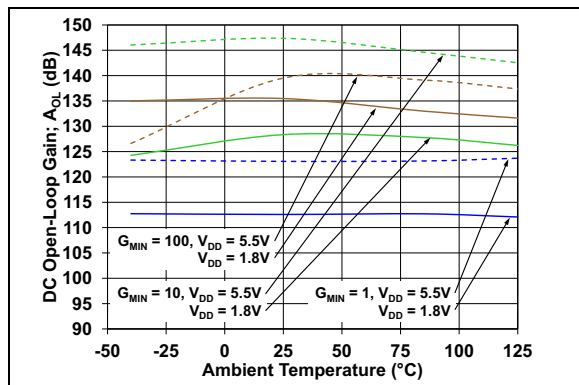
FIGURE 2-43: DC Open-Loop Gain vs. Ambient Temperature.
