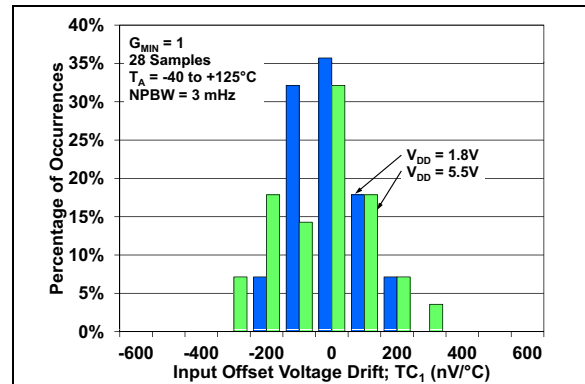
FIGURE 2-4: Input Offset Voltage Drift, with G_{MIN} = 1 .
