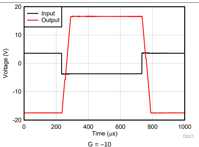
Figure 28. Overload Recovery
