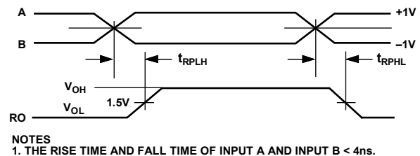
Figure 13. Receiver Propagation Delays
