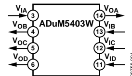
Figure 4. ADuM5403W
