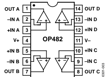
Figure 3. 14-Lead PDIP (P-Suffix) [IN-14]
