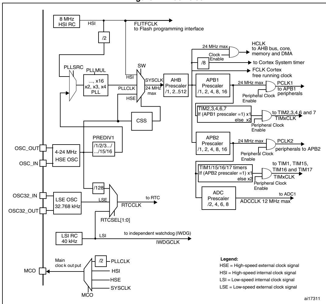
Figure 2. Clock tree
