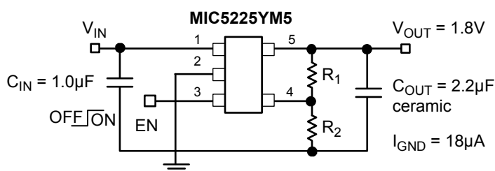
Ultra-Low Current Adjustable Regulator Application
