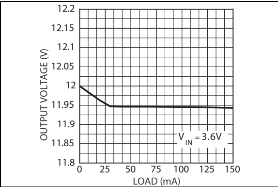
FIGURE 2-2: Load Regulation.
