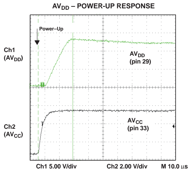
Figure 46. Power-Up Response
