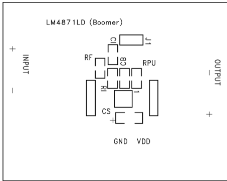
Figure 28. Recommended NGN PC Board Layout: Component-Side Silkscreen
